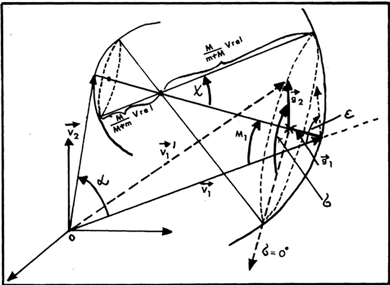
Energy transfer in elastic collisions
