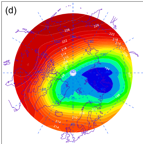
LS temperature, day 50, year 2016
