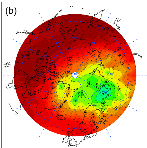
Column ozone, day 50, year 2016
