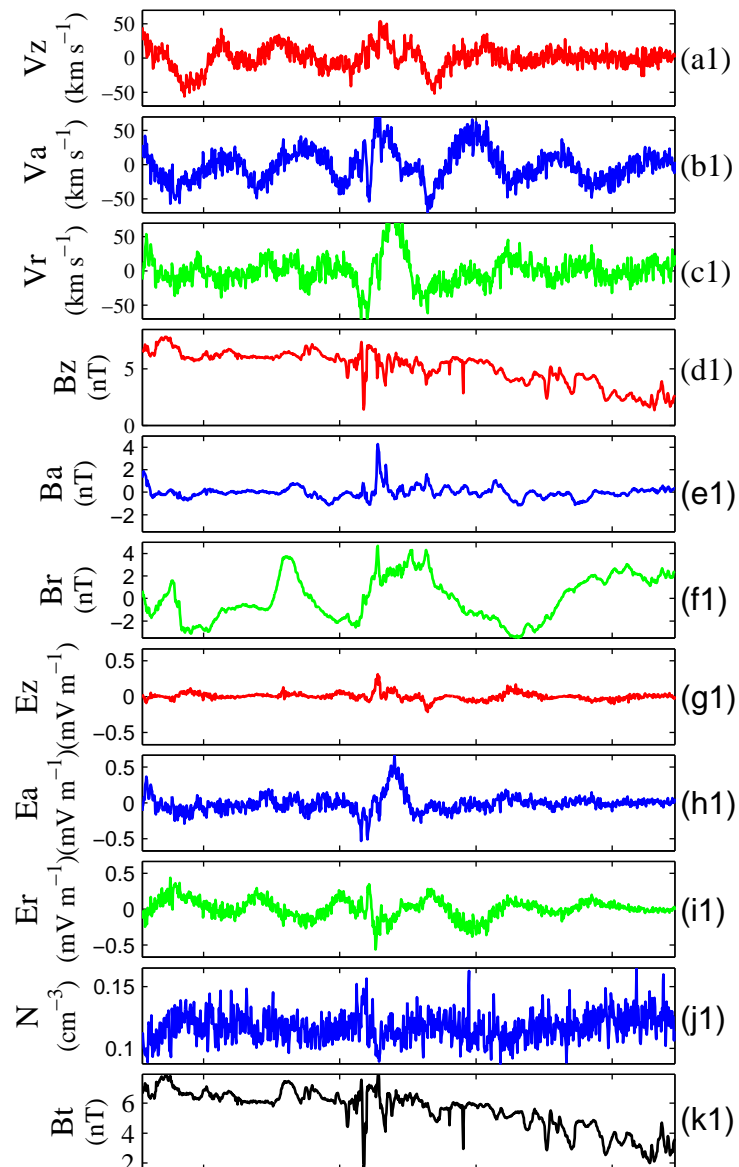
Event A (THEMIS-c 01-Feb-2009)
