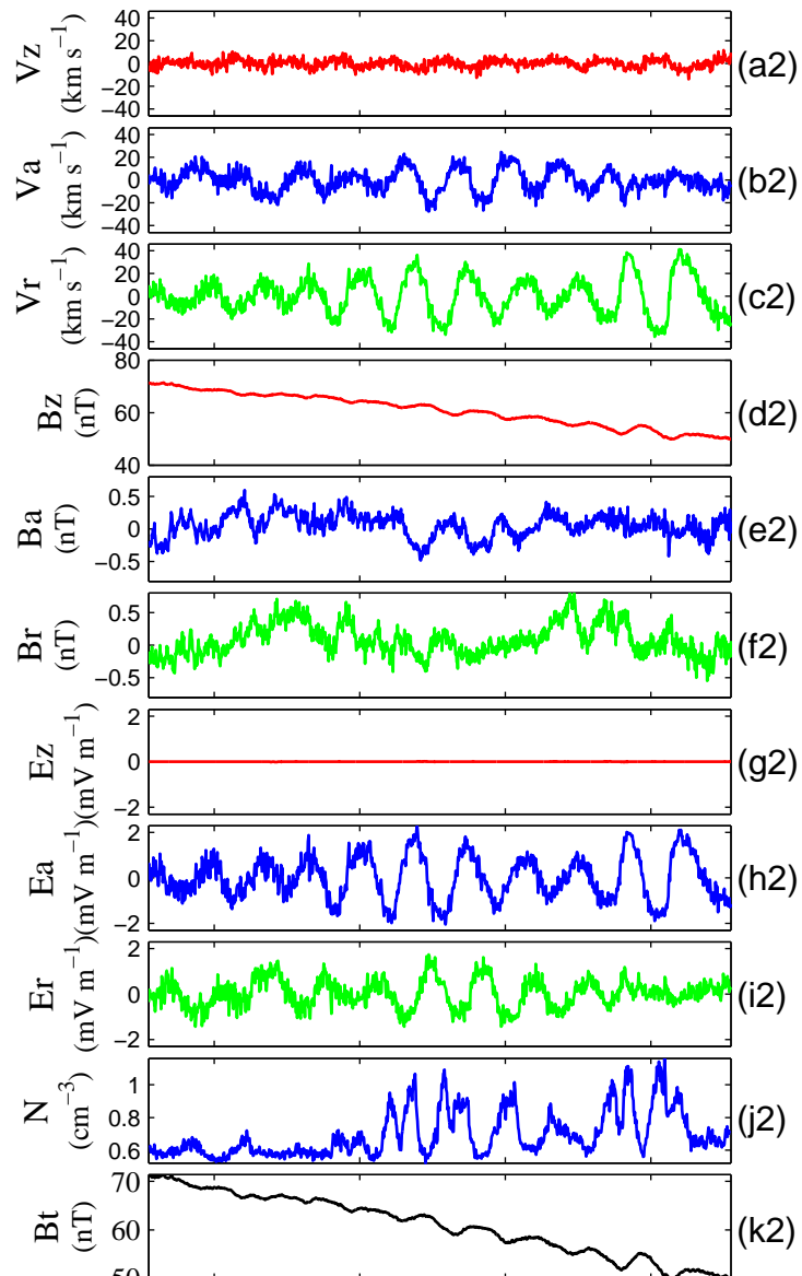
Event B (THEMIS-a 11-Apr-2013)
