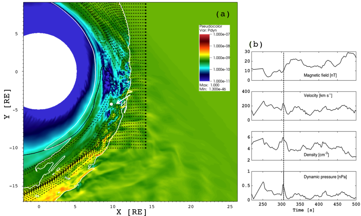
Figure 1. (a) Dynamic pressure within the Vlasior simulation domain. Bow shock position is identified with white solid line. The black dashed lines are solar wind streamlines illustrating the magnetopause position roughly (see text for details). The figure is a snapshot of Supplement movie S1, which does not include the bow shock position or the streamlines. The arrow indicates the visually detected magnetosheath jet under scrutiny in this paper. (b) Virtual spacecraft data from the location marked with a white dot in panel (a): magnetic field, velocity, density, and dynamic pressure as a function of time. The dashed vertical line shows the time of the visually identified jet in panel (a).
