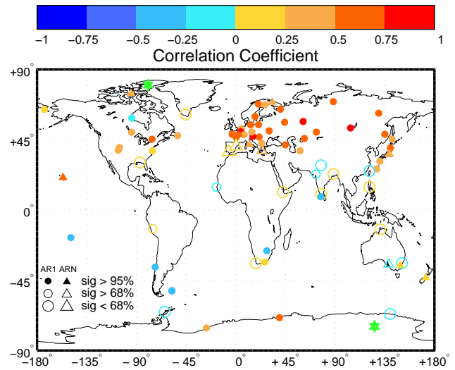
Figure 2. Correlation coefficients for log power ratios of semi-annual to annual variability in f_oF_2 for each station compared with Slough/Chilton. Each correlation is represented by a symbol plotted at the location of the ionospheric monitoring station. Positive correlations are shown in colours ranging from yellow to red while negative correlations are shown as shades of blue. Correlations exceeding 95 % significance are represented by filled symbols; correlations that are less significant than this are represented by open circles according to the scale shown. Circles represent correlations for which only the first lag of the autocorrelation function needed to be accounted for; triangles represent correlations where more than one lag needed to be accounted for. The positions of the geomagnetic poles are indicated by green stars.
