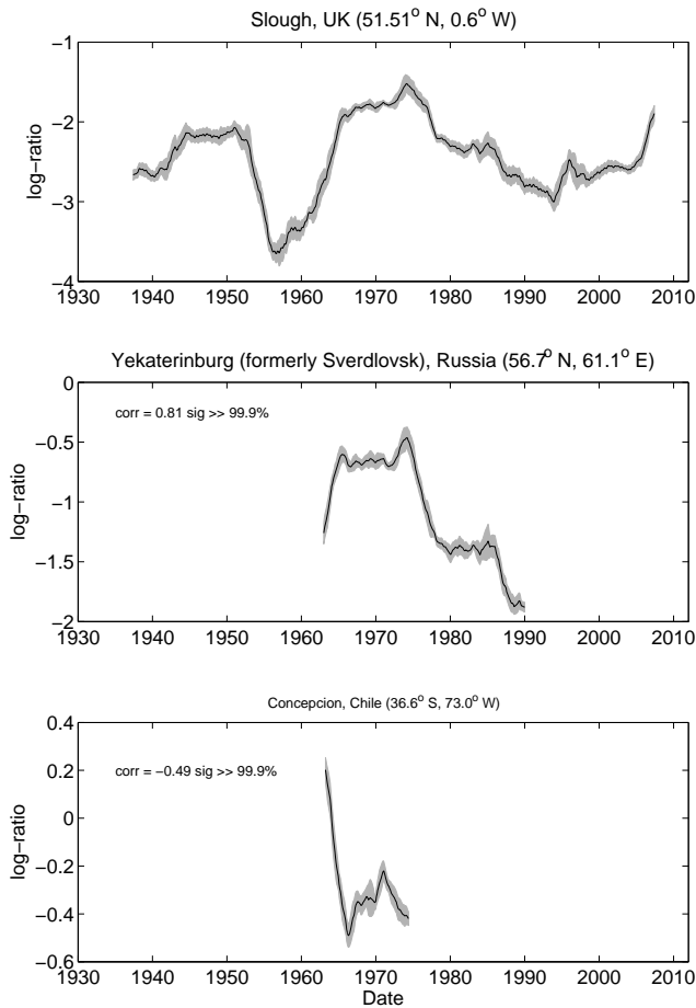
Figure 1. Log power ratios of the semi-annual to annual components of noon median values of f_oF_2 (black lines) against time for three ionospheric monitoring stations; Slough/Chilton (top), Sverdlovsk (middle) and Concepción (bottom). The standard error for each station is shown as a grey band around the black line. For the two lower panels, the value and significance of the correlation with Slough is shown.
