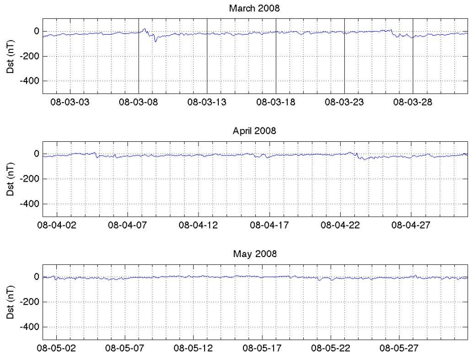
Fig. 4. Variation of Dst for the period 1 March 2008 until 31 May showing the magnetic activity of the magnetosphere for the period around the time of occurrence of the Sichuan earthquake (12 May 2008).
