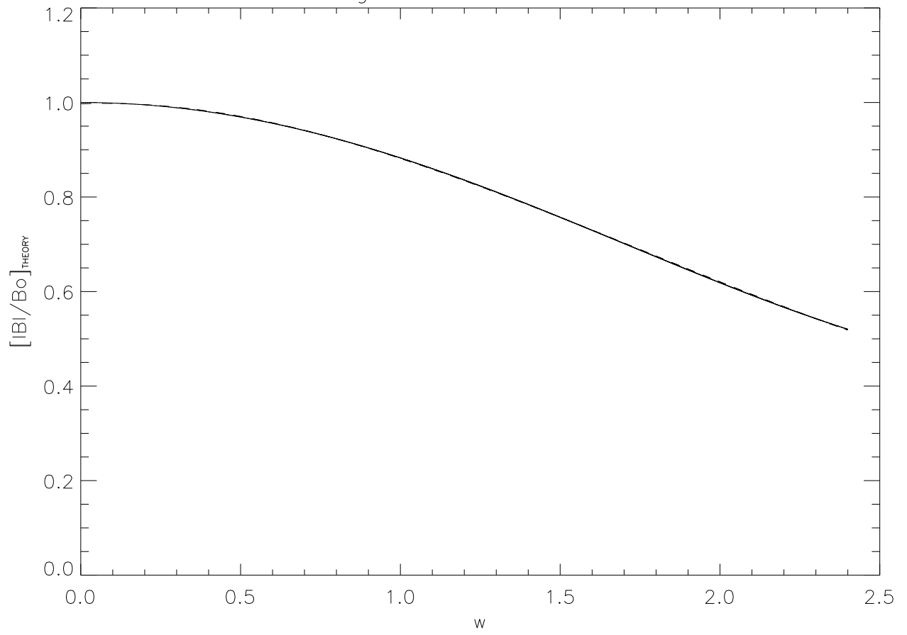
Magnitude of Bessel Field
