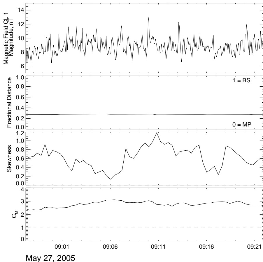
Fig. 7. Observations of magnetic peaks by Cluster 1 on 27 May 2005 (same panels as in Fig. 1).
