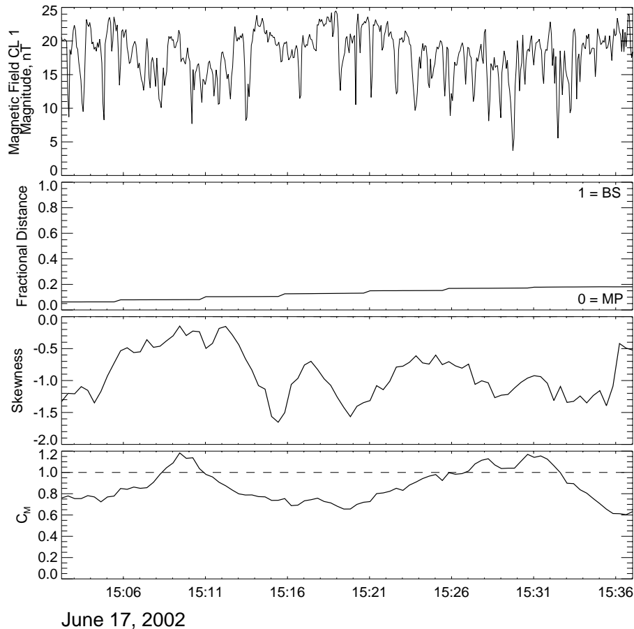
Fig. 6. Observations of magnetic holes by Cluster 1 on 17 June 2002 (same panels as in Fig. 1).
