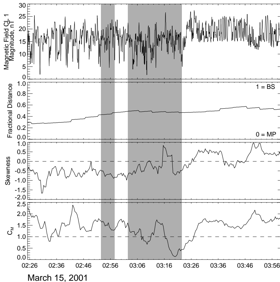
Fig. 2. Observations of mirror structures by Cluster 1 on 15 March 2001. From top to bottom: magnetic field amplitude, fractional distance F , skewness of magnetic fluctuations and mirror parameter C_M . The grey color codes windows of 5 min when mirror structures are not detected by the algorithm based on magnetic fluctuations.
