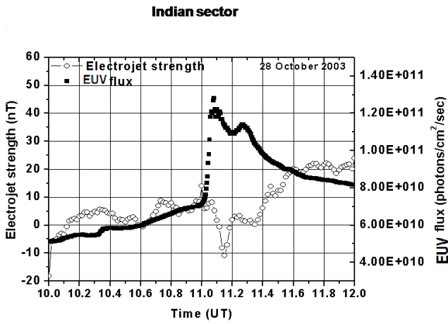
Fig. 6a. The time variations of EUV flux and electrojet strength at the station of Trivandrum ( 77^\circ E) on 28 October 2003.
