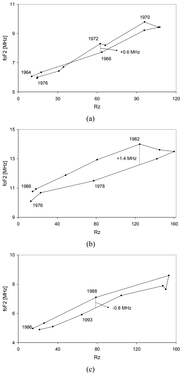
Fig. 1. Monthly median f_oF2 at noon in terms of R_z for (a) Mundaring in September during solar cycle 20 (b) Ahmadabad in April during solar cycle 21 and (c) Argentine Islands in April during solar cycle 22. The vertical dashed line indicate the maximum amplitude of the hysteresis which is given in MHz.
