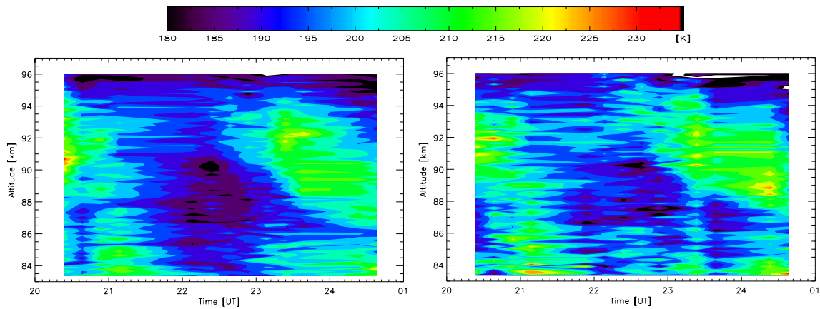
Fig. 7. Contour plots of 15 min averaged temperatures from the ALOMAR Weber Na lidar on 5–6 November 2005. Beam 1 (left) is pointing 20° W of zenith. Beam 2 (right) is pointing 20° E of zenith.
