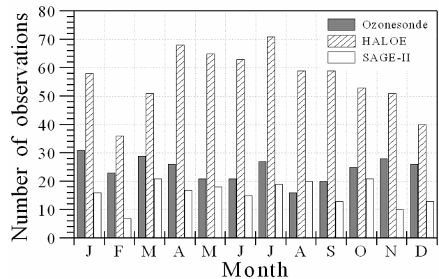
Fig. 1. Histogram represents the monthly distribution of ozonesonde, HALOE and SAGE-II satellite data used for the present study and for the period from 1992 to 2005.
