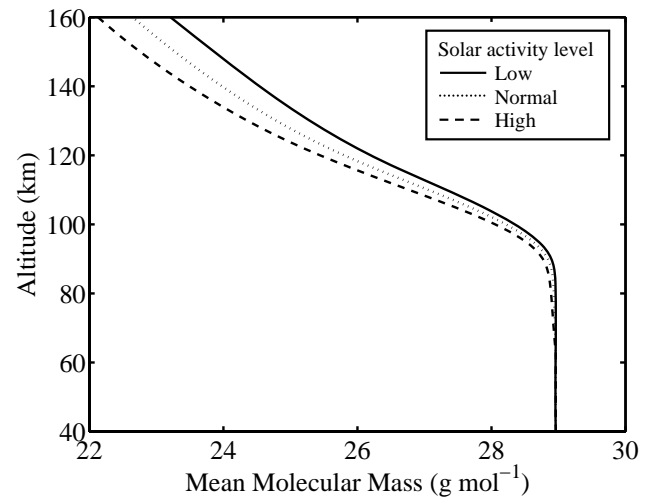
Fig. 2. Mean molecular mass as a function of altitude.
