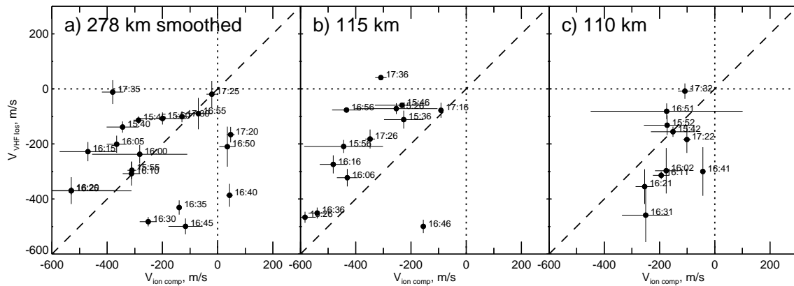
Fig. 4. Scatter plots of line-of-sight irregularity drift velocity measured by the STARE Finland radar in beam 4 and bin 24, V_{VHF\ los} , against the component of the EISCAT ion drift velocity resolved along the STARE beam 4 direction at (a) 278, (b) 115, and (c) 110 km. The time (interval centre) of measurements is indicated near each point.
