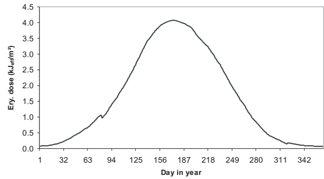
Fig. 3. Climatic annual cycle of the clear-weather daily erythemal dose in \text{kJ}_{ef}/\text{m}^2 for Tartu-Tõravere Meteorological Station site.
