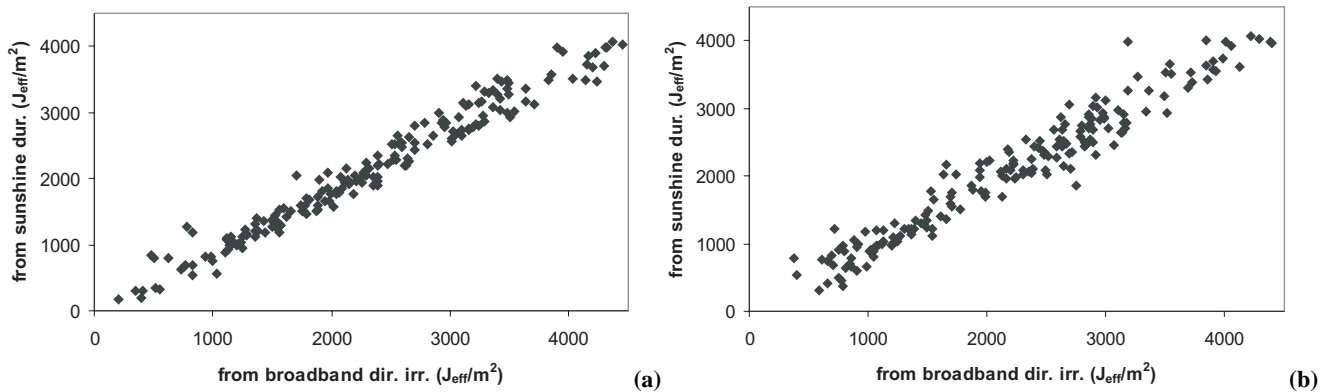
Fig. 9. Comparison of reconstructed daily erythemal doses based on broadband direct irradiance and on sunshine duration in summer half-year of normal atmospheric transparency 1999 (a) and in summer half-year with soot aerosol episodes 2002 (b).
