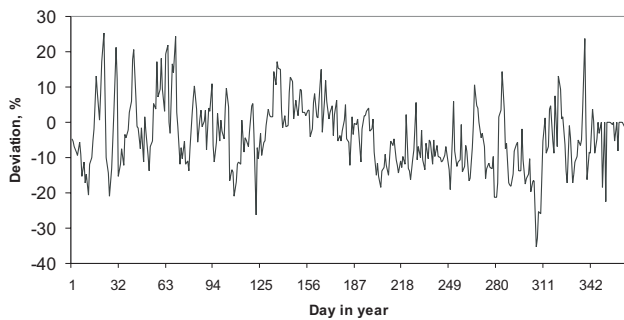
Fig. 4. Daily percent deviations of total ozone from its climatic value in year 2004 at Tartu-Tõravere Meteorological Station site.
