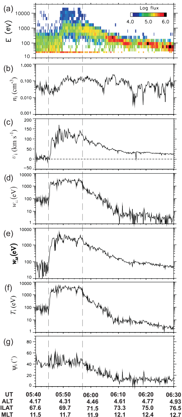
Fig. 3. Overview of a transverse O + ion heating event on 28 September 2001, between 05:40 and 06:30 UT: (a) time-energy spectrogram of O + ions, (b) O + ion density in cm -3 , (c) upward mean velocity in km s -1 , (d) perpendicular mean energy in eV, (e) parallel mean energy in eV, (f) temperature in eV, and (g) apex angle in °. The vertical dashed lines indicate the boundaries of the heating region.
