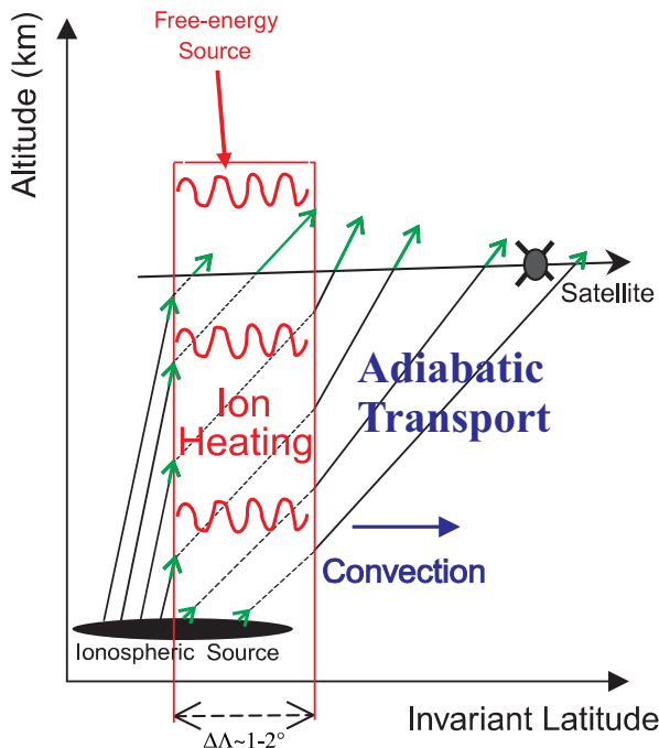
Fig. 1. Two-dimensional (invariant latitude-altitude) sketch that illustrates the transport patterns of ion outflows from an ionospheric source of finite latitudinal extent \Delta\Lambda throughout the cusp/cleft and dayside polar cap, in conjunction with a high-altitude satellite pass. The green vectors correspond to the ion velocities and their lengths are proportional to their intensities.
