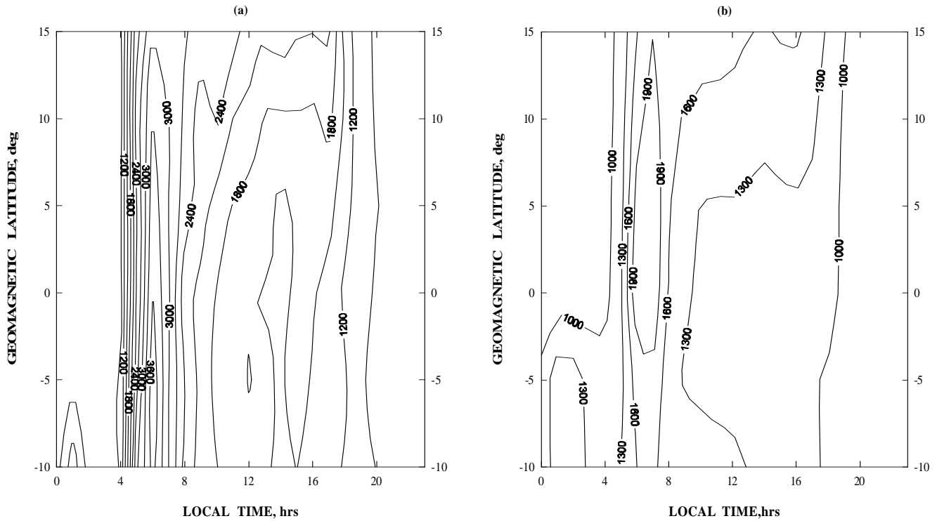
Fig. 4. Latitudinal and diurnal variation of electron temperature at ~500 km for (a) observed (b) IRI in northern winter.
