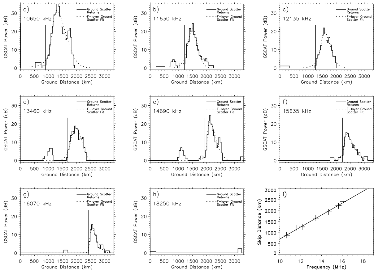
Fig. 1. (a)–(h) Ground-scatter as a function of range from the Kodiak SuperDARN radar observed on 23 June 2001 between 22:40 and 22:55 UT. The solid vertical lines in each panel show the F-region skip distance. (i) F-region skip distances identified in (a)–(h) plotted as a function of frequency. The solid line is a linear least-squares fit to these data.
