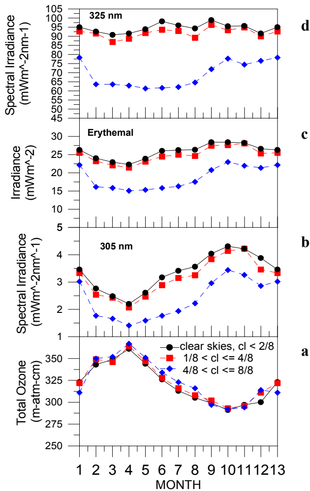
Fig. 1. The annual cycle of (a) total ozone, (b) solar spectral irradiance at 305 nm, (c) erythemal irradiance, and (d) solar irradiance at 325 nm under different sky conditions at 63^\circ SZA as derived from measurements performed at Thessaloniki between November 1990 and November 1997.
