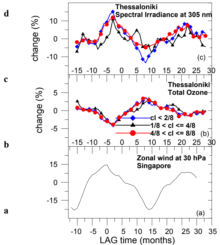
Fig. 2. Composites of (a) 30 hPa zonal wind at Singapore, (b) total ozone at Thessaloniki, and (c) solar irradiance at 305 nm. The composites have been calculated for the last four QBO cycles (1990–1997) and measurements correspond to all-sky conditions and a solar zenith angle of 63^\circ .
