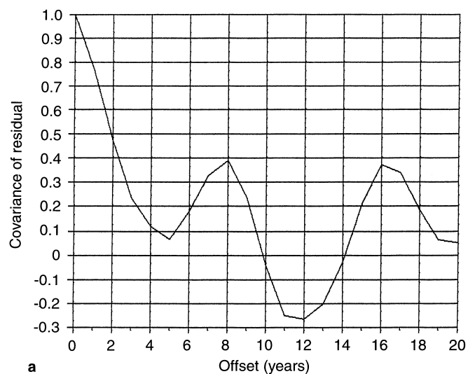
Fig. 10a. Covariance of residual
